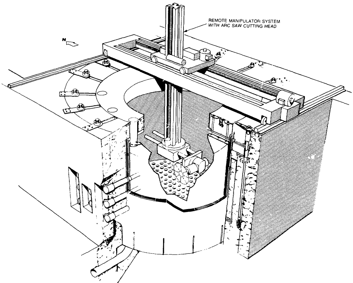
FIGURE 3 CALANDRIA AND THERMAL SHIELD VESSEL SECTIONING
