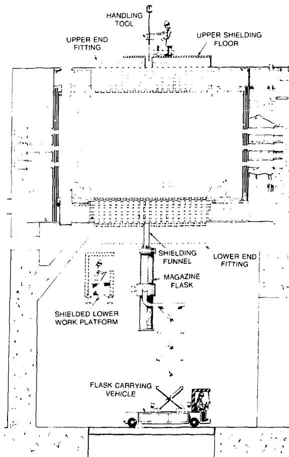
FIGURE 2 FUEL CHANNEL REMOVAL
